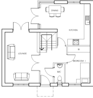
GROUND FLOOR PLAN PLOTS 24,25,27
