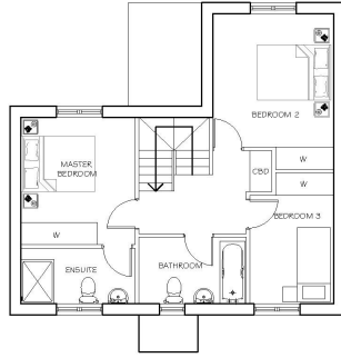
FIRST FLOOR PLAN PLOTS 24,25,27
