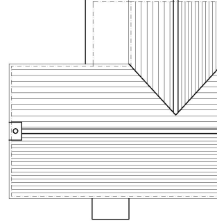
ROOF PLAN PLOTS 24,25,27
